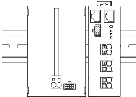
Mount UPS upside down
